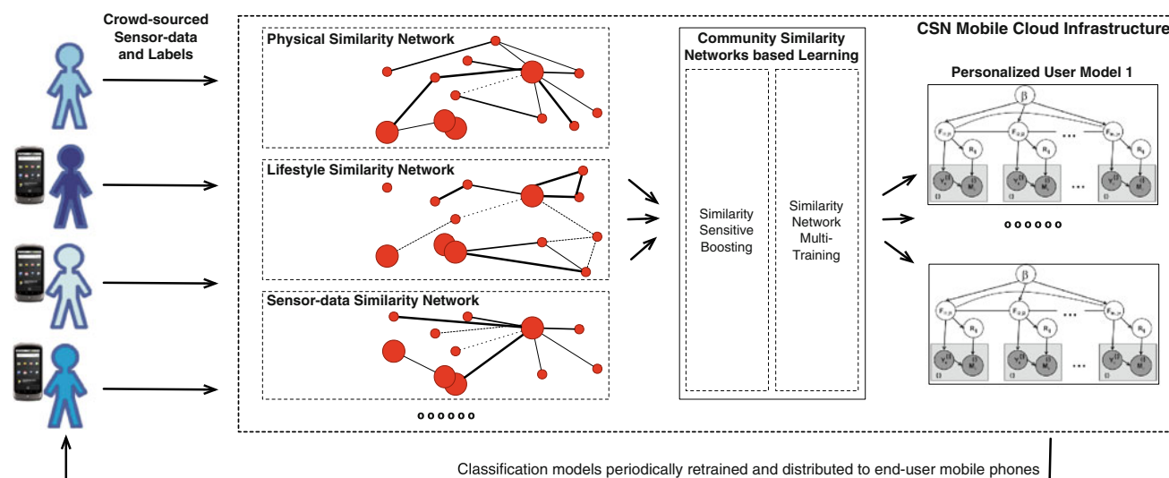
Fig. 3 The processing phases within Community Similarity Networks
