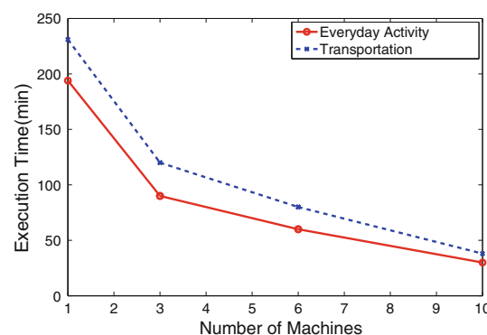
Fig. 9 Latency of processing training data decreases as the pool of cloud nodes is increased
